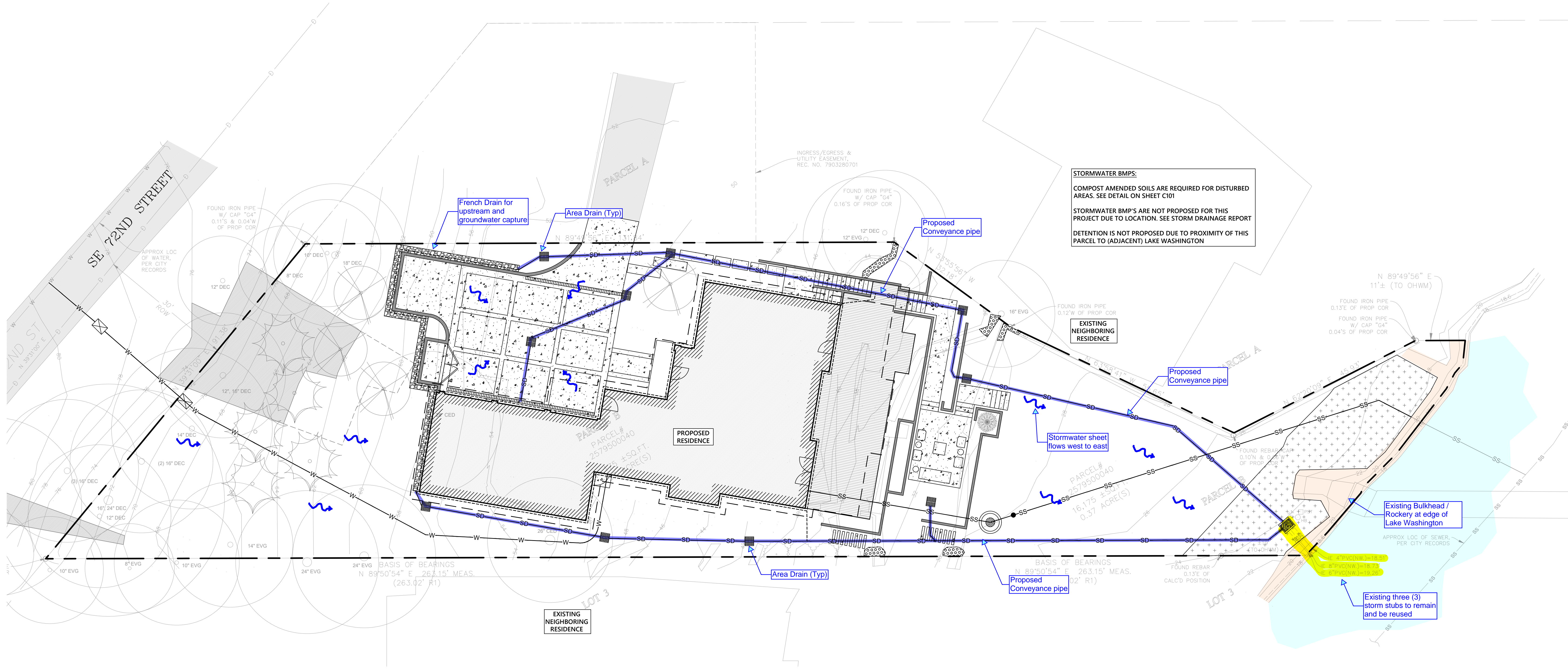
FIGURE 6 - PROPOSED CONDITIONS
